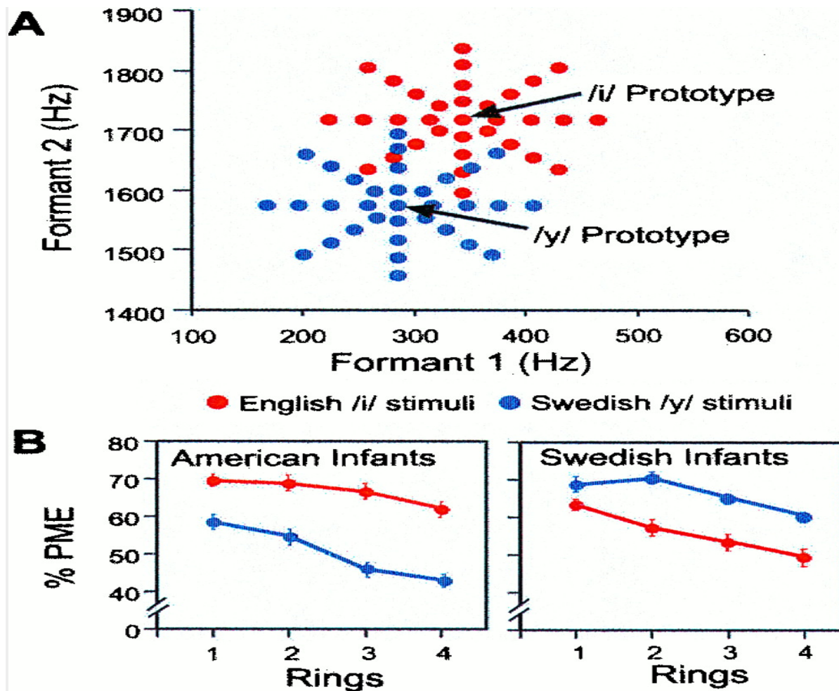
A) Formant frequencies of vowels surrounding an American/i/prototype (red) and a Swedish/y/prototype (blue). B) Results of tests on American and Swedish infants indicating an effect of linguistic experience. Infants showed greater generalization when tested with native-language prototype. PME = Perceptual magnet effect (Kuhl 2000a).
